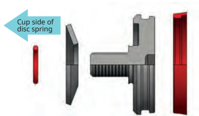
1x Disc Spring C100 Compact- C250 Compact
